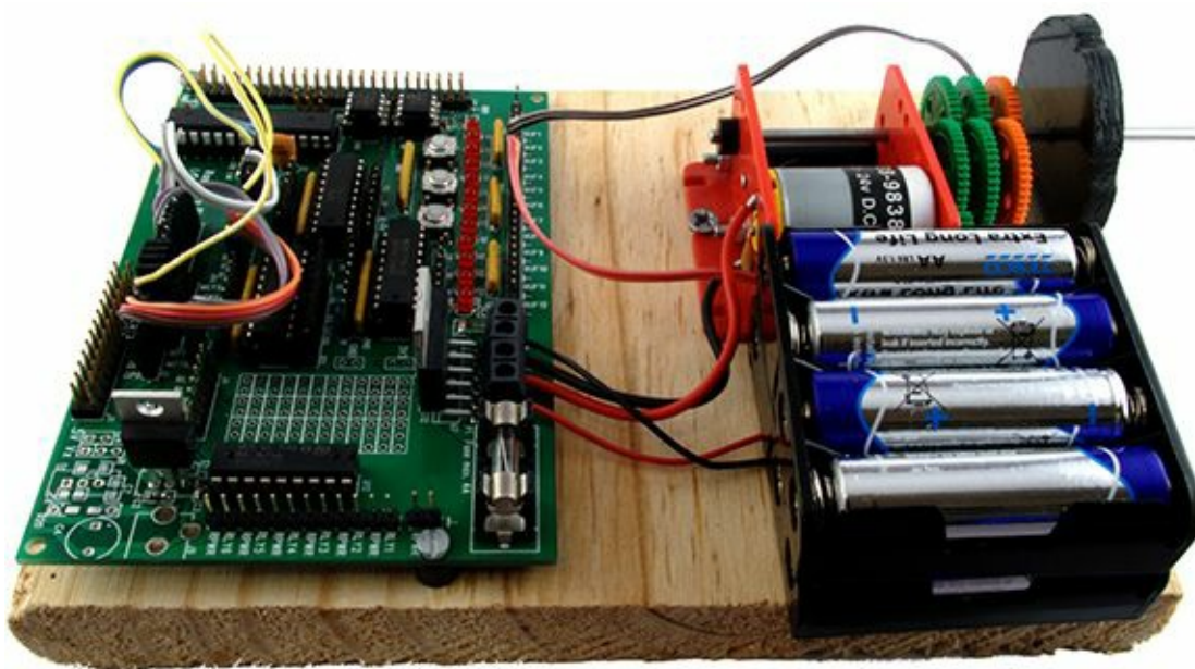
Figure 13-9: Using the Gertboard motor controller
