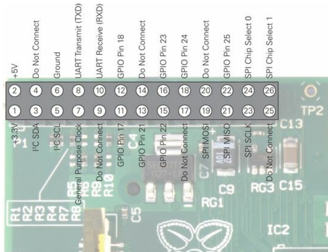
Figure 12-2: The Raspberry Pi’s GPIO port and its pin definitions
