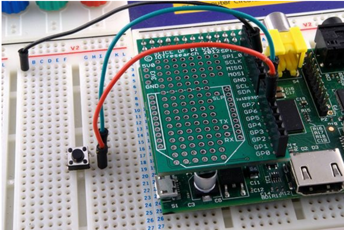
Figure 13-2: Connecting the Slice of Pi to a breadboard
