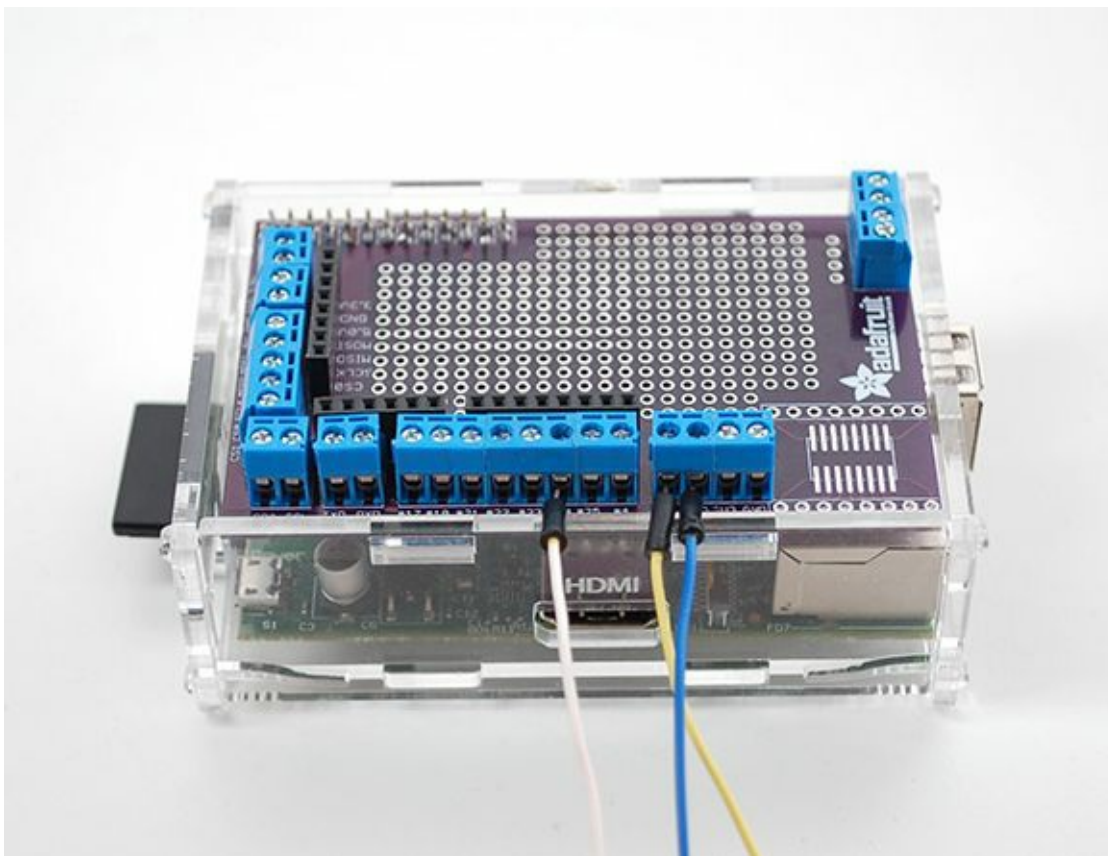
Figure 13-6: The Pi Plate connected to a cased Raspberry Pi
