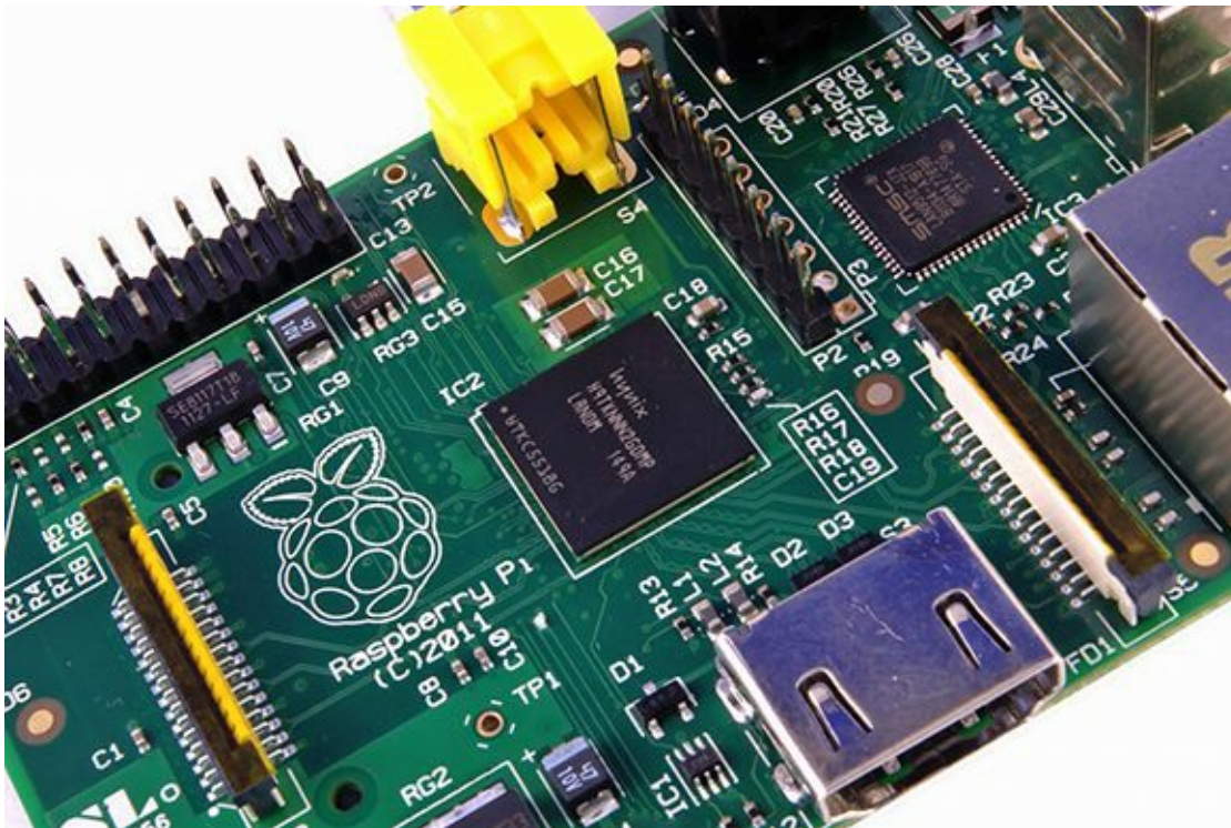
Figure 1-1: The BCM2835 SoC, located beneath a Hynix memory chip
