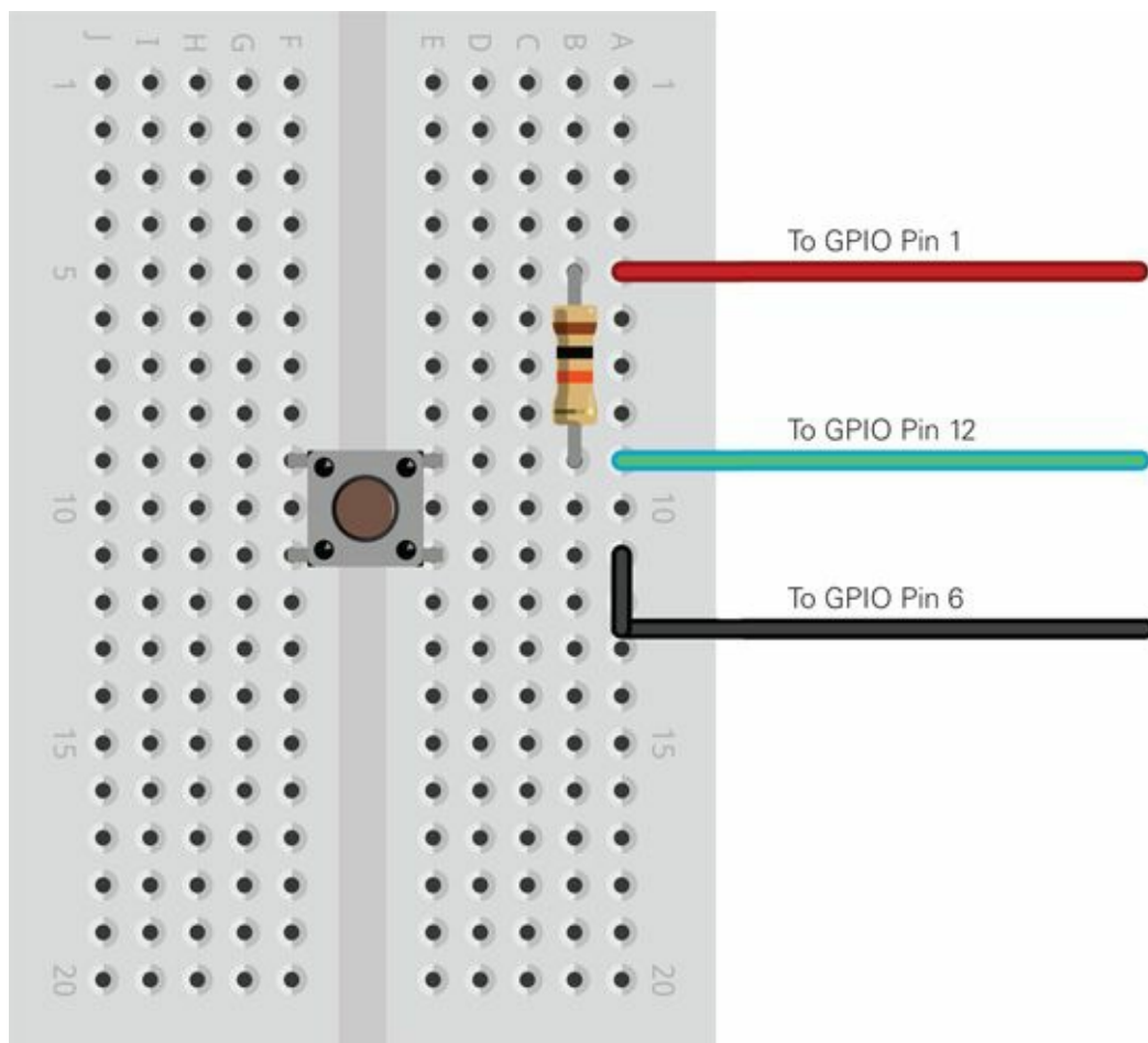
Figure 12-5: The example breadboard layout for a simple push-button input
