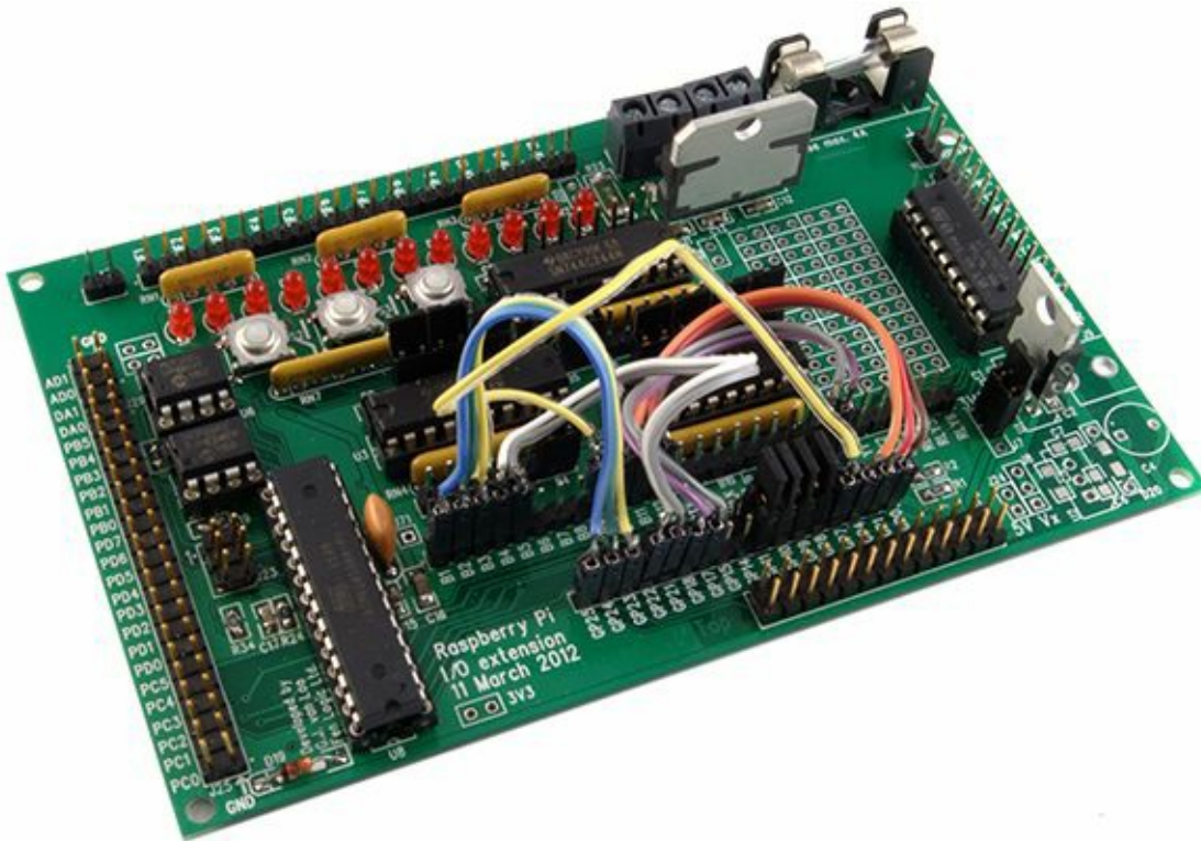
Figure 13-7: The Gertboard, designed by Gert van Loo
