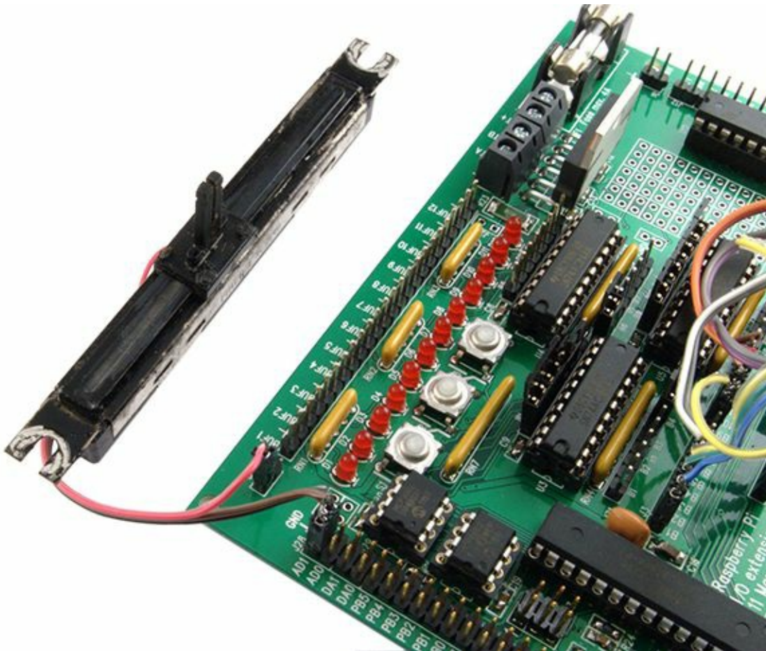
Figure 13-10: Connecting a potentiometer to the Gertboard's ADC pins
